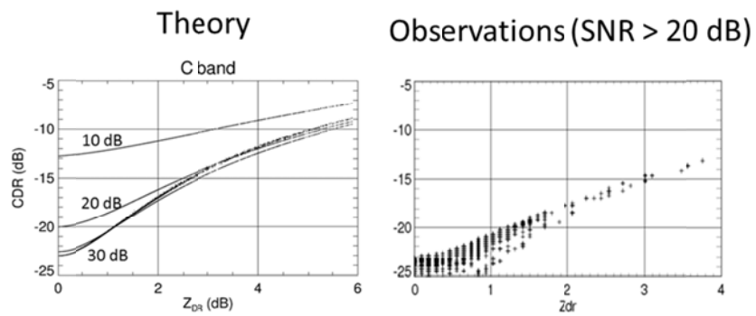
Fig. 5. (a) Theoretical dependencies of measured CDR on Z_{DR} in rain for different values of SNR; (b) scatterplot of measured CDR vs Z_{DR} in rain on 28 January 2014.
